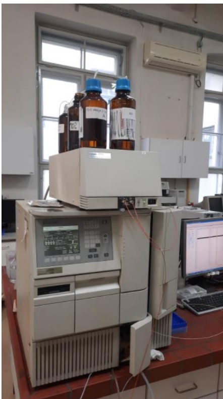
Figure 30. Waters 2795 Alliance HPLC system with 2996 PDA detector
