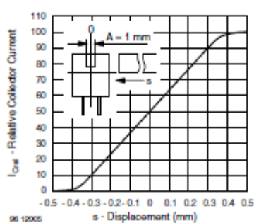
Fig. 11 - Relative Collector Current vs. Displacement
