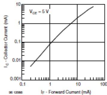
Fig. 7 - Collector Current vs. Forward Current
