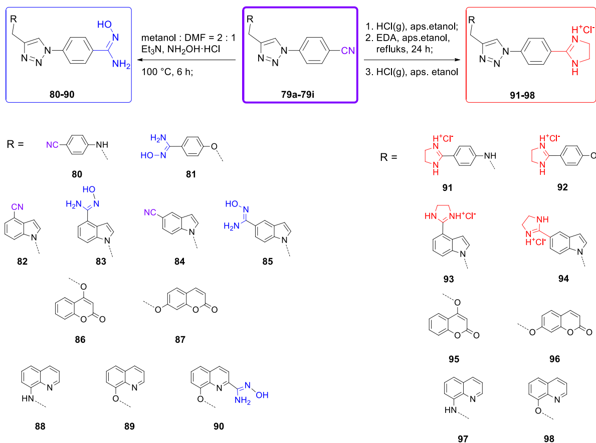
Shema 19. Sinteza amidoksim- ( 80-90 ) i amidino-supstituiranih derivata ( 91-98 ) 1,2,3-triazola
