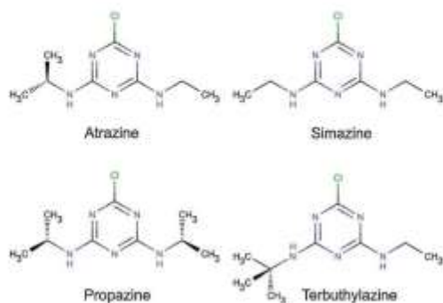
Fig. 1. Schematic representation of terbuthylazine structure ( N - tert -butyl-6-chloro- N -ethyl-1,3,5-triazine-2,4-diamine) and other representatives of s -triazine herbicides.
