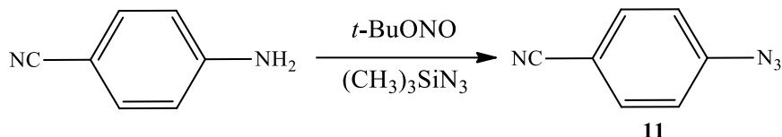
Shema 4. Sinteza 4-azidobenzonitrila ( 11 )
