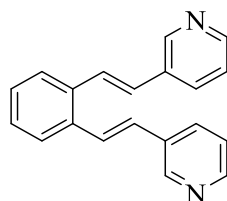
trans,trans-1
