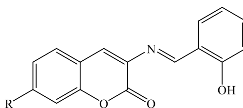
13a R = OH 13b R = \text{NEt}_2
