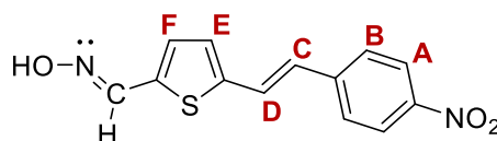
trans, syn-19
