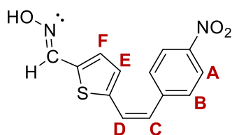
cis, syn-19
