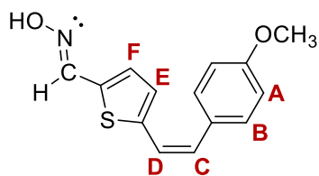
cis, syn-16
