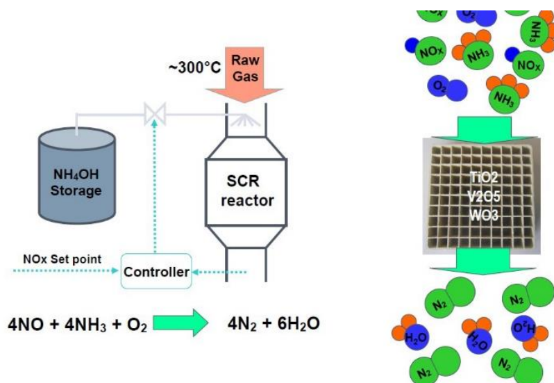
Figure 12. The mechanism of SCR performance for NO x abatement [10]
