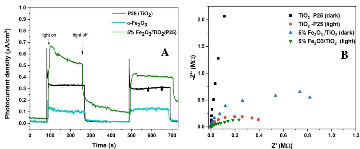
Figure 46. (A) Transient photocurrent responses of \text{TiO}_2 -P25, \alpha\text{-Fe}_2\text{O}_3 , and 5% (w/w) \text{Fe}_2\text{O}_3/\text{TiO}_2 nanocomposites, and (B) EIS Nyquist plots of \text{TiO}_2 -P25 and 5% (w/w) \text{Fe}_2\text{O}_3/\text{TiO}_2 in dark and light conditions
