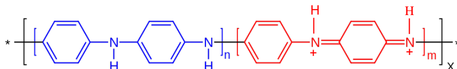
Slika 4.42. Strukturna formula molekule PANI polimera; benzenoidne i kinoidne jedinice, [(-\text{B}-\text{NH}-\text{B}-\text{NH}-)_x(-\text{B}-\text{N}=\text{Q}=\text{N}-)]_m
