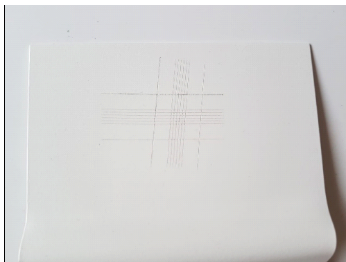
Figure 59: Adhesion test result of the sample PA7 before adding adhesion promoter (BYK-4510); the result is B4
