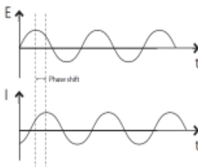
Figure 37: Sinusoidal current response in a linear system
