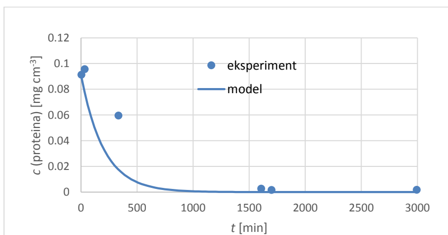
Slika 27. Sinteza Zn nanočestica (redistirana voda, c(\text{NaNO}_3) = 0,1 \text{ M} , T = 25^\circ\text{C} , 150 rpm, c_{\text{ureaze}} = 1 \text{ mg cm}^{-3} , c_{\text{uree}} = 3,33 \text{ mM} , c(\text{Zn}(\text{NO}_3)_2) = 1 \text{ mM} , V = 5 \text{ cm}^3 ), vremenska ovisnost koncentracije proteina
