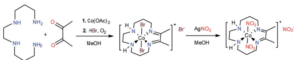
Slika 6. Shema sinteze [\text{Co}(\text{DIM})\text{Br}_2]^+ i [\text{Co}(\text{DIM})(\text{NO}_3)_2]^+ [11]
