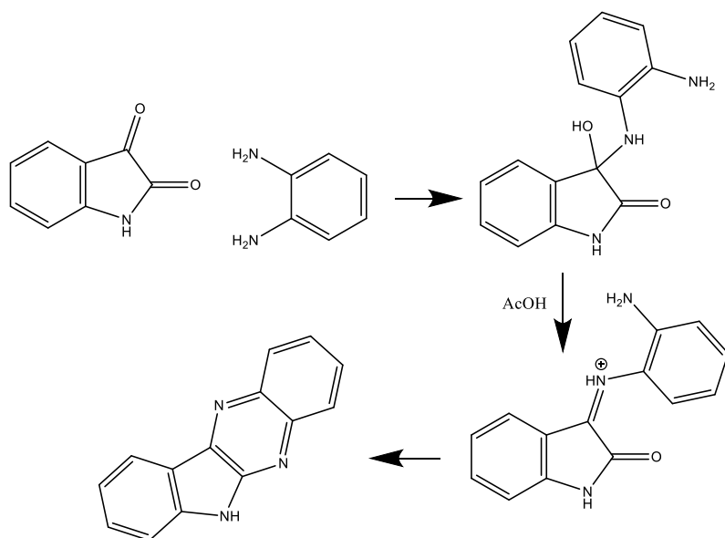
HEMA 3: Sinteza 6H-indolo[2,3-b]kinoksalina (3)
