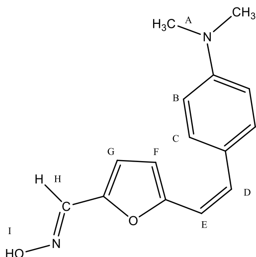
cis,syn-9
