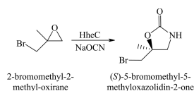
Scheme 16. Synthesis of ( S )-5-bromomethyl-5-methylloxazolidin-2-one catalysed by HheC. [51]
