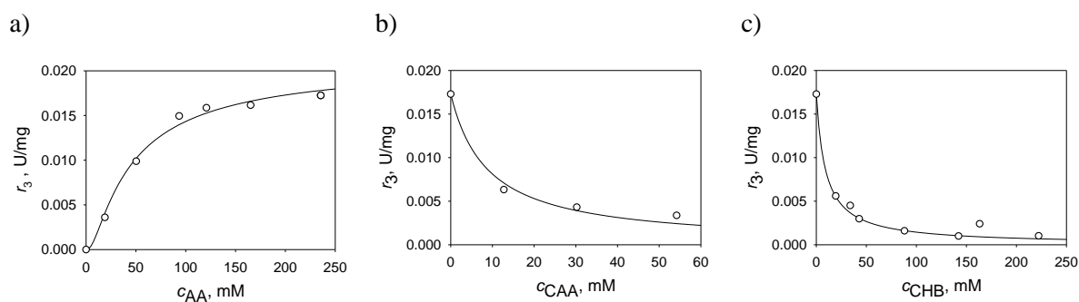
Figure 36 Kinetics of the DERA 024 -catalyzed AA self-aldol addition (0.1 M phosphate buffer pH 6, \mu_{\text{DERA}} = 1 mg/mL, 1 000 rpm, 25 °C). The dependence of the initial reaction rate on a) AA, b) CAA ( c_{\text{AA}} = 200 mM) and c) CHB ( c_{\text{AA}} = 200 mM). Legend: experiment (dots), model (line).
