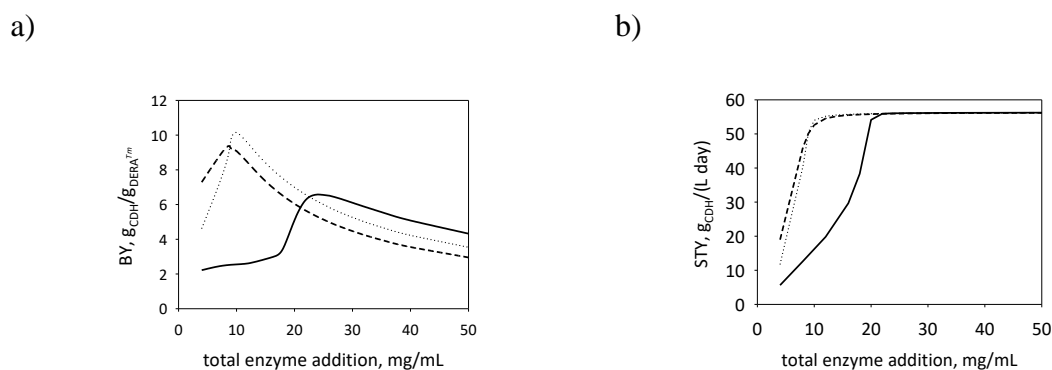
Figure 50 Model simulations of the double aldol addition of AA to CAA catalyzed by DERA Tm in different fed-batch reactor modes (feed 1: q_1 = 5 \mu\text{L}/\text{min} ; c_{AA,0} = 2300 \text{ mM} , c_{CAA,0} = 950 \text{ mM} , FBR1 and FBR2: V_0 = 6 \text{ mL} ; feed 2: q_2 = 2 \mu\text{L}/\text{min} ; FBR3: V_0 = 10 \text{ mL} ). a) Biocatalyst yield and b) productivity change with total enzyme addition. Legend: FBR1 (solid line), FBR2 (dotted line), FBR3 (dashed line).
