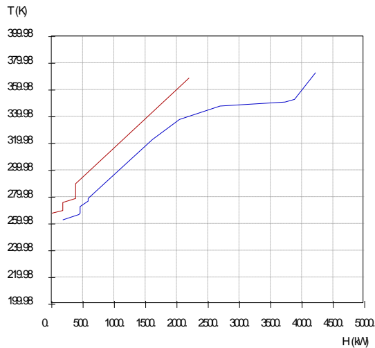
Composite Curves
