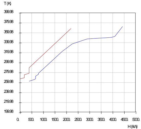
Composite Curves
