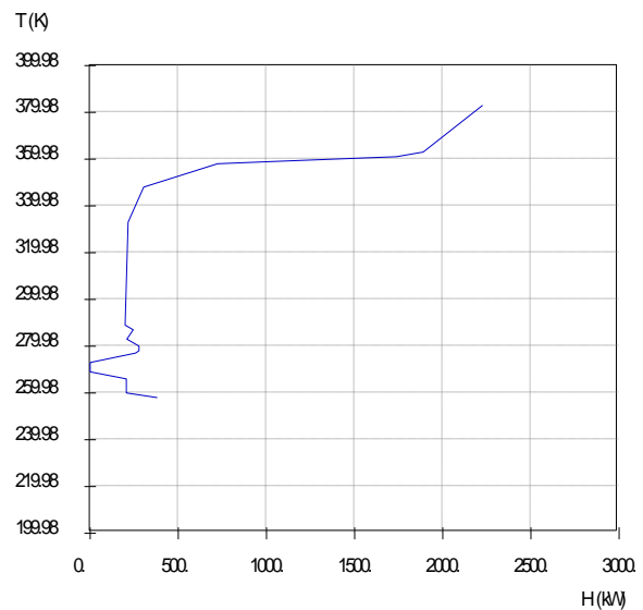
Grand Composite Curve
