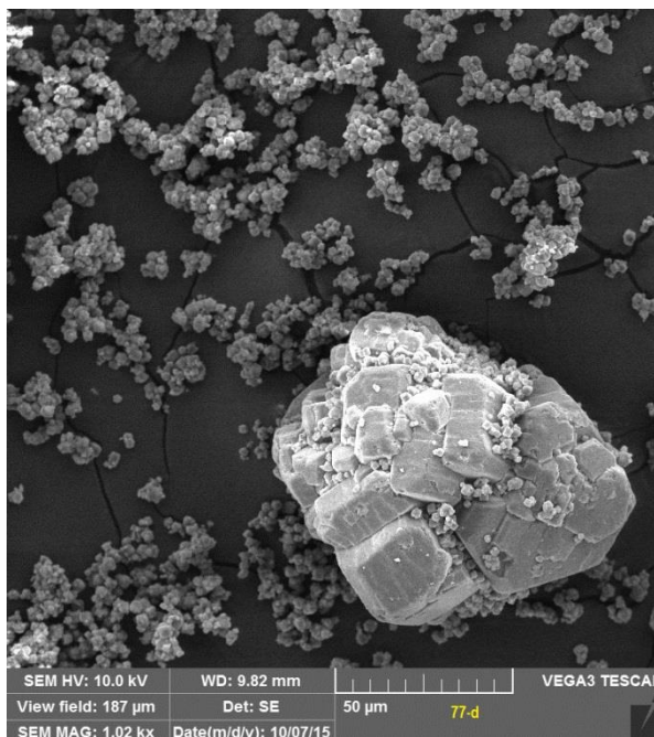
d) \text{Al}_2\text{O}_3 + \text{MCC Na} (1000 \times )
