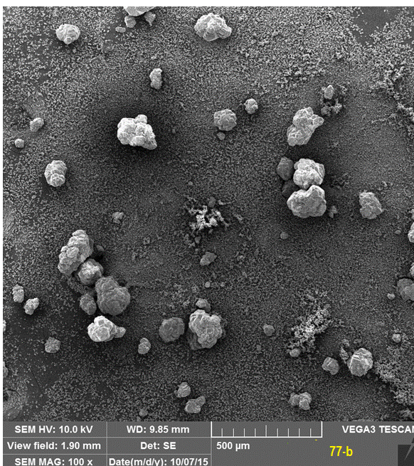
b) \text{Al}_2\text{O}_3 + \text{MCC Na} + 2\text{-CEES} (100 \times )
