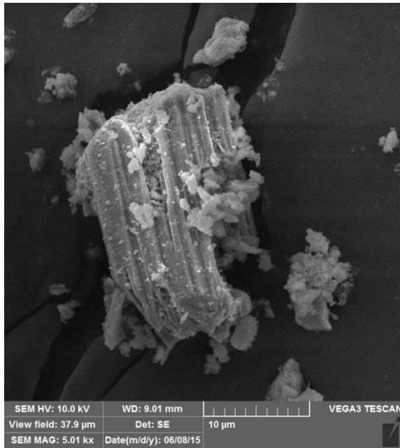
c) Klinoptilolit (5000 ×)
