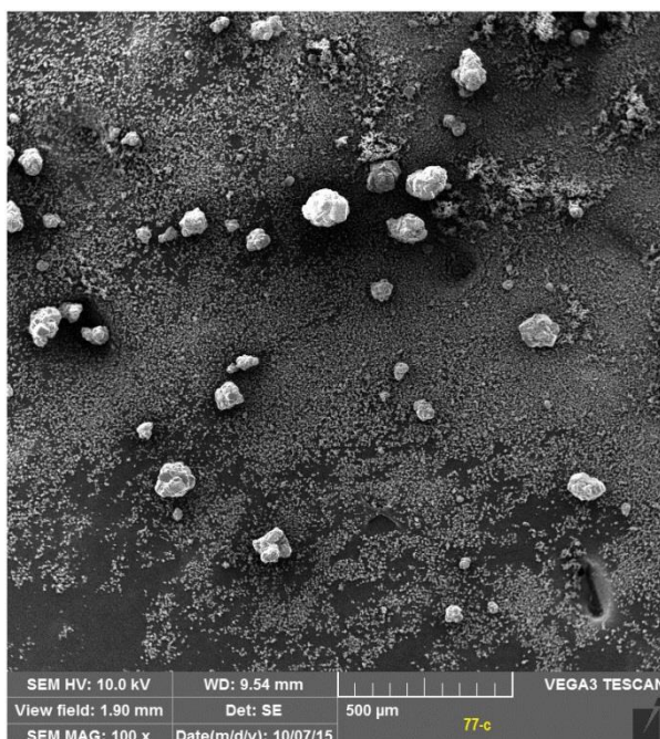
c) \text{Al}_2\text{O}_3 + \text{MCC Na} + \text{DMMP} (100 \times )
