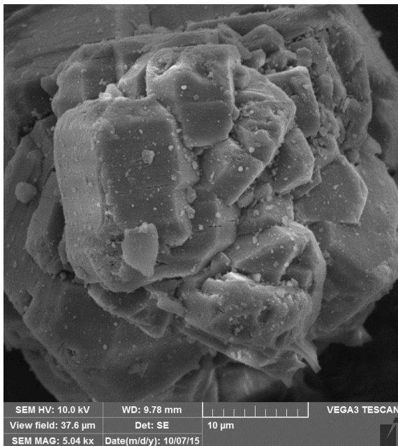
g) \text{Al}_2\text{O}_3 (5000 ×)
