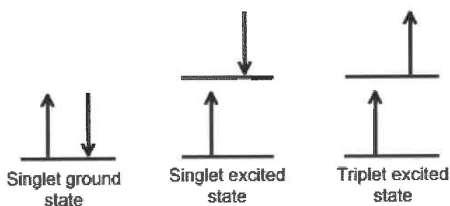
Figure 4 Singlet and triplet energy levels.
