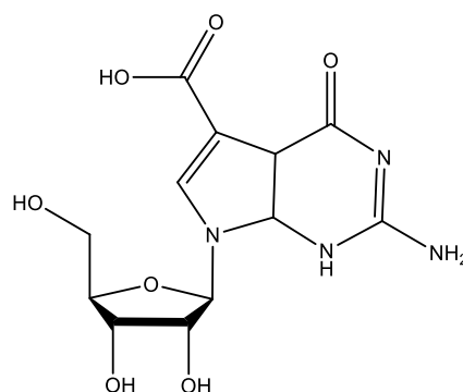
kadeguomicin
