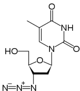
azidotimidin
