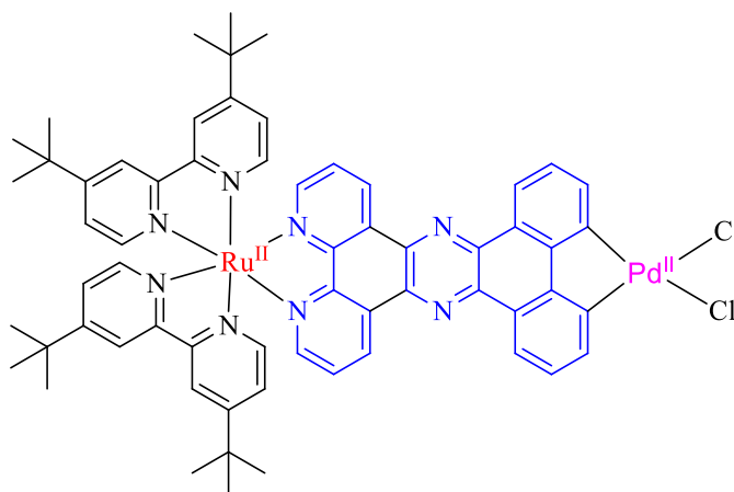
Slika 2.14 Monomolekularni fotokatalizator \text{Ru}(\text{tpphz})\text{Pd} (tpphz – tetrapirido[3,2-a:2',3'-c:3'',2''-h;2''',3'''-j]fenazin)
